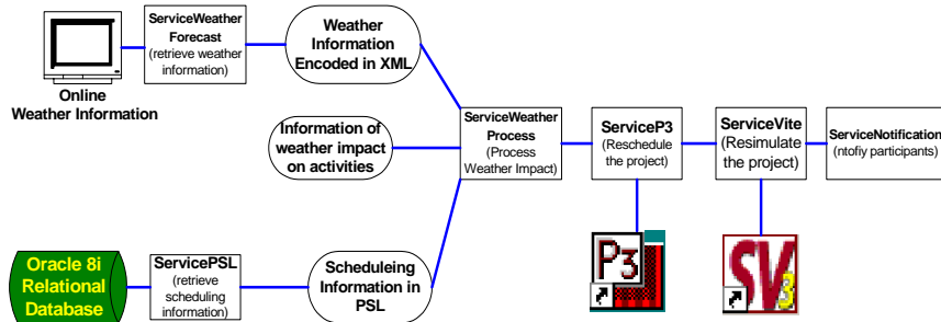
Figure 8: The Workflow in the Weather Demonstration
