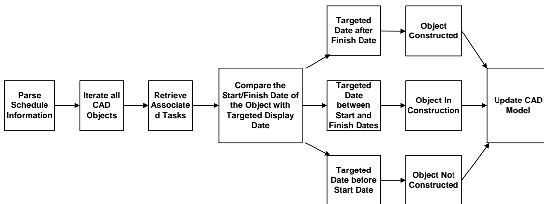
Figure 3: Process for Integrating Project Schedule and CAD Model Display
